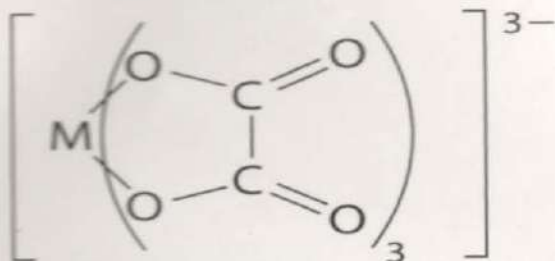
Oxalate ion
