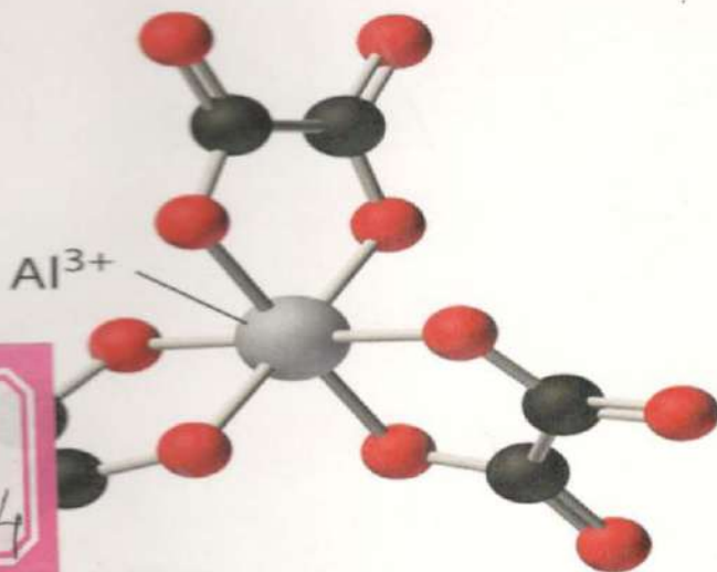
\text{Al}^{3+} -oxalate complex
